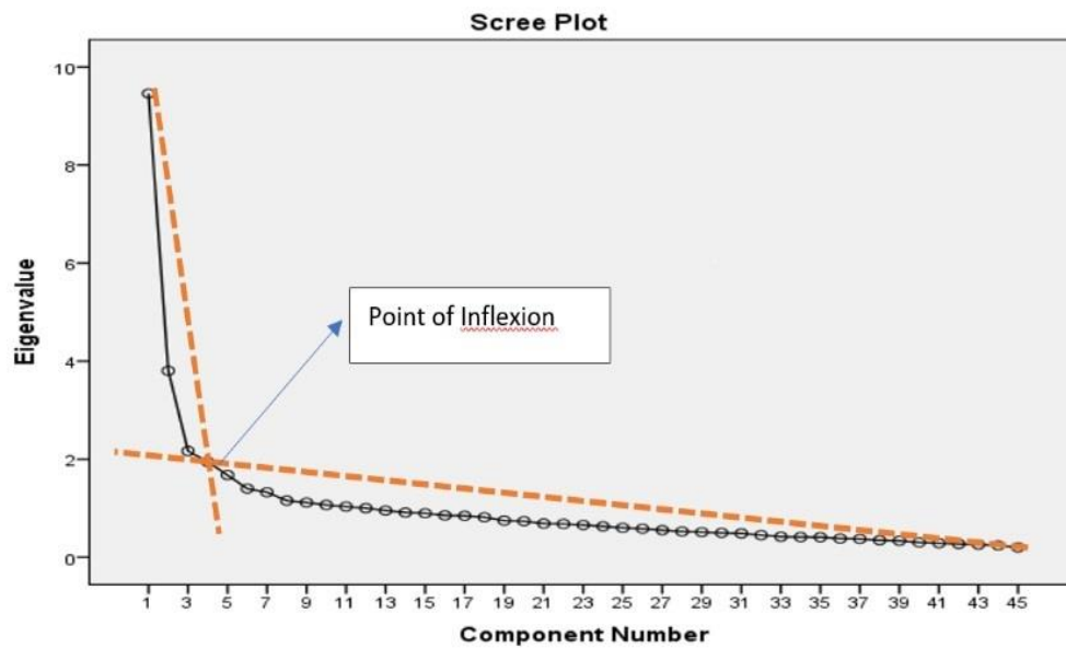
Figure 1. Scree Plot
